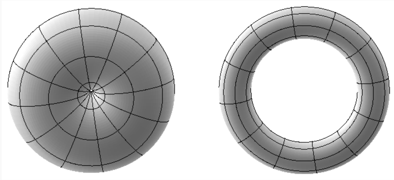
Figure 9-6 : Texture-Map Distortion
